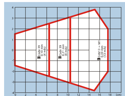
Reading zone (15° skew angle)
